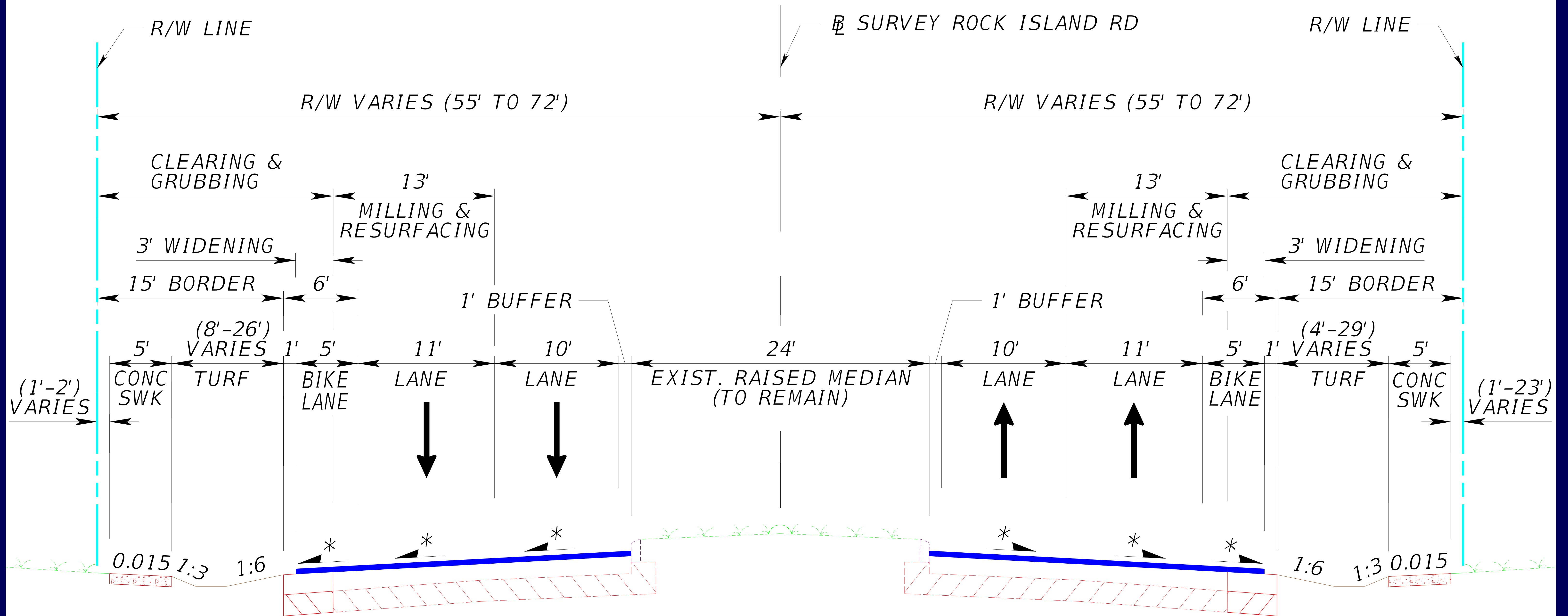
TYPICAL SECTION ROCK ISLAND RD. W. SAMPLE RD. TO WILES RD.
